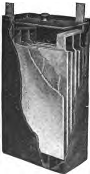
FIG. 453.—One Cell of the "Gould" Storage Battery for Electric Vehicle Use. According to the data given by the manufacturers, this cell, containing four negative and three positive plates, has a normal charging rate of 27 amperes; a discharge rate of 2\frac{3}{4} amperes for 4 hours; a capacity of 81 ampere-hours at 3 hours' discharge, and of 90 ampere-hours at 4 hours' discharge. The plates are each 5\frac{1}{8} \times 7\frac{3}{4} inches, and the total dimensions of the cell, enclosed in its rubber jar, are 2\frac{1}{2} \times 6\frac{1}{4} \times 11 inches. Forty such cells are generally used for an average light vehicle battery.
